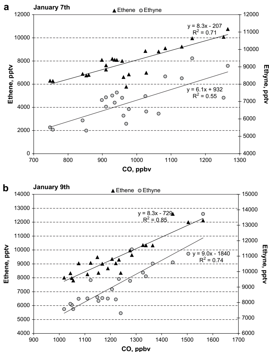
Fig. 5. CO versus ethene and ethyne for (a) January 7th and (b) January 9th, 2004. An exceptionally high ethyne mixing ratio measured on January 7th was excluded from the overall correlation (11 ppbv), while one exceptionally high mixing ratio of CO was excluded on January 9th (2.2 ppmv).
