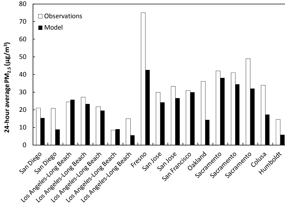
Figure 36: Modeled and observed 24-hour average PM 2.5 concentrations for December 7, 2005 at selected locations
