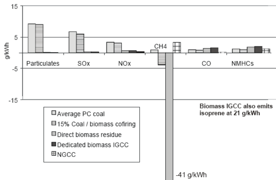
Figure 16: Life cycle pollutant emissions for several different scenarios of electricity generation (Bain et al., 2003)
