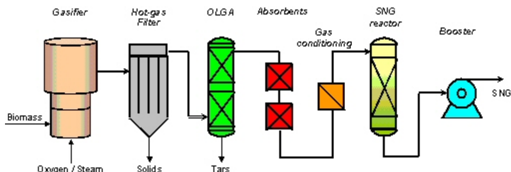
Figure 22: Schematic of RSNG production from biomass through gasification and methanation (Zwart et al. 2006). This example includes a stage for tar removal using a proprietary technology called OLGA.
