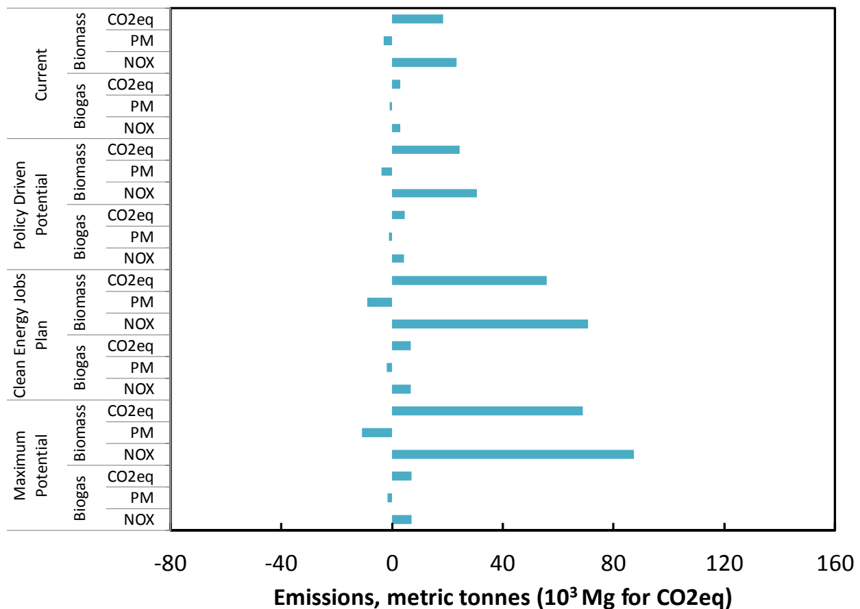
Figure 26: Net emissions from biomass in scenarios with current biomass technology (group A)
