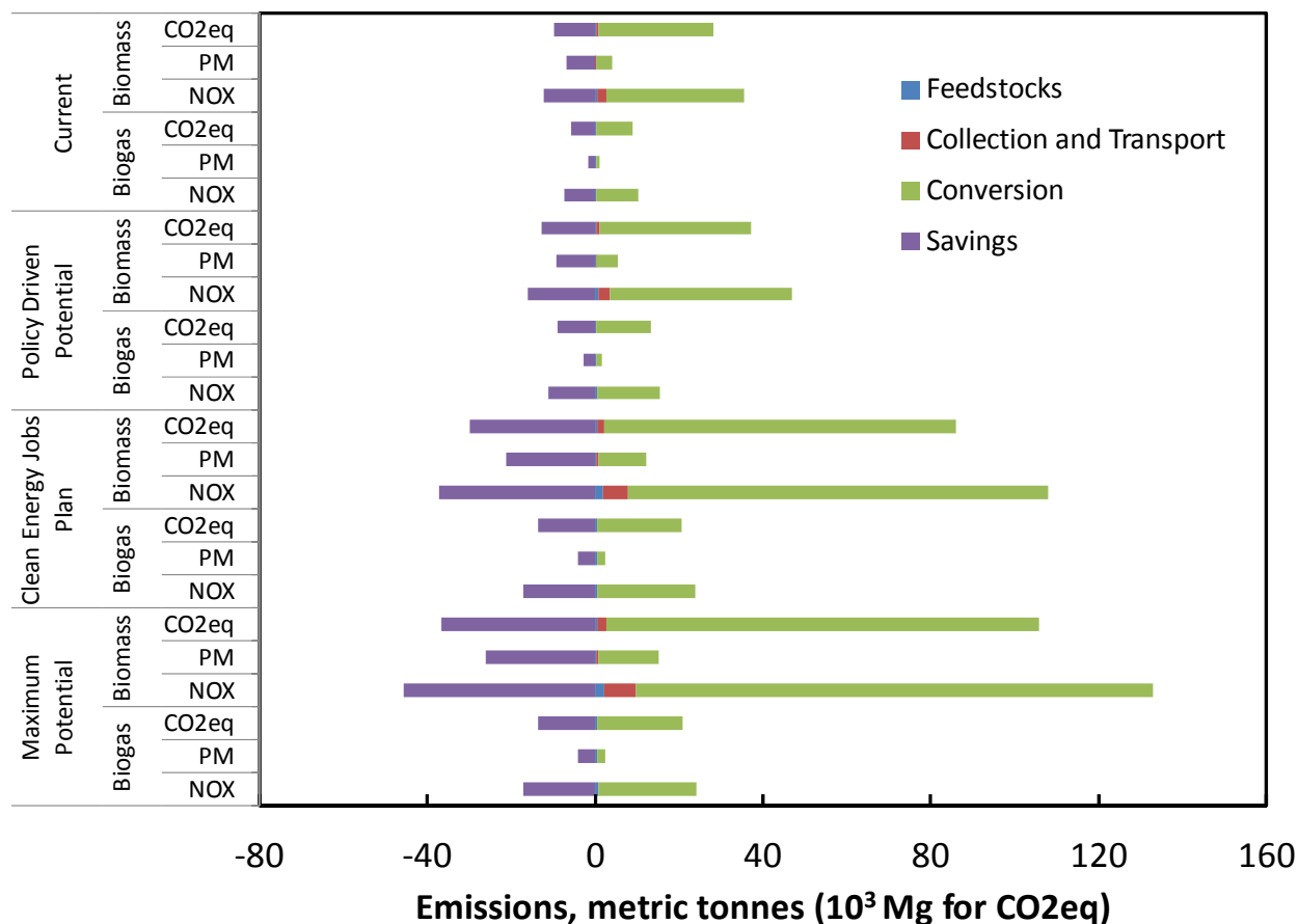
Figure 25: Summary of emissions from biomass in scenarios with current biomass technology (group A)
