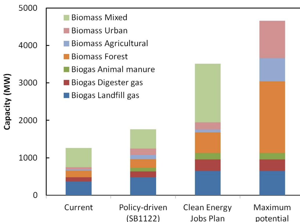
Figure 24: Summary of power generation capacity from biomass scenarios with current biomass technology estimated for the year 2020
