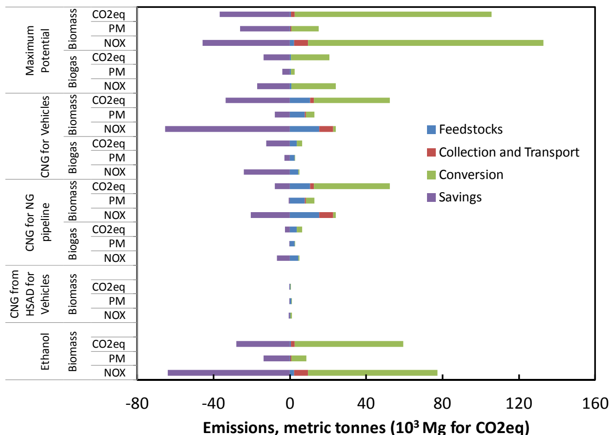
Figure 29: Comparison of emissions from biomass in scenarios with maximum biomass potential using current technology for biopower (group A) and scenarios with a shift end use from electricity to fuel (group C-1, C-2, C-3 and C-4)
