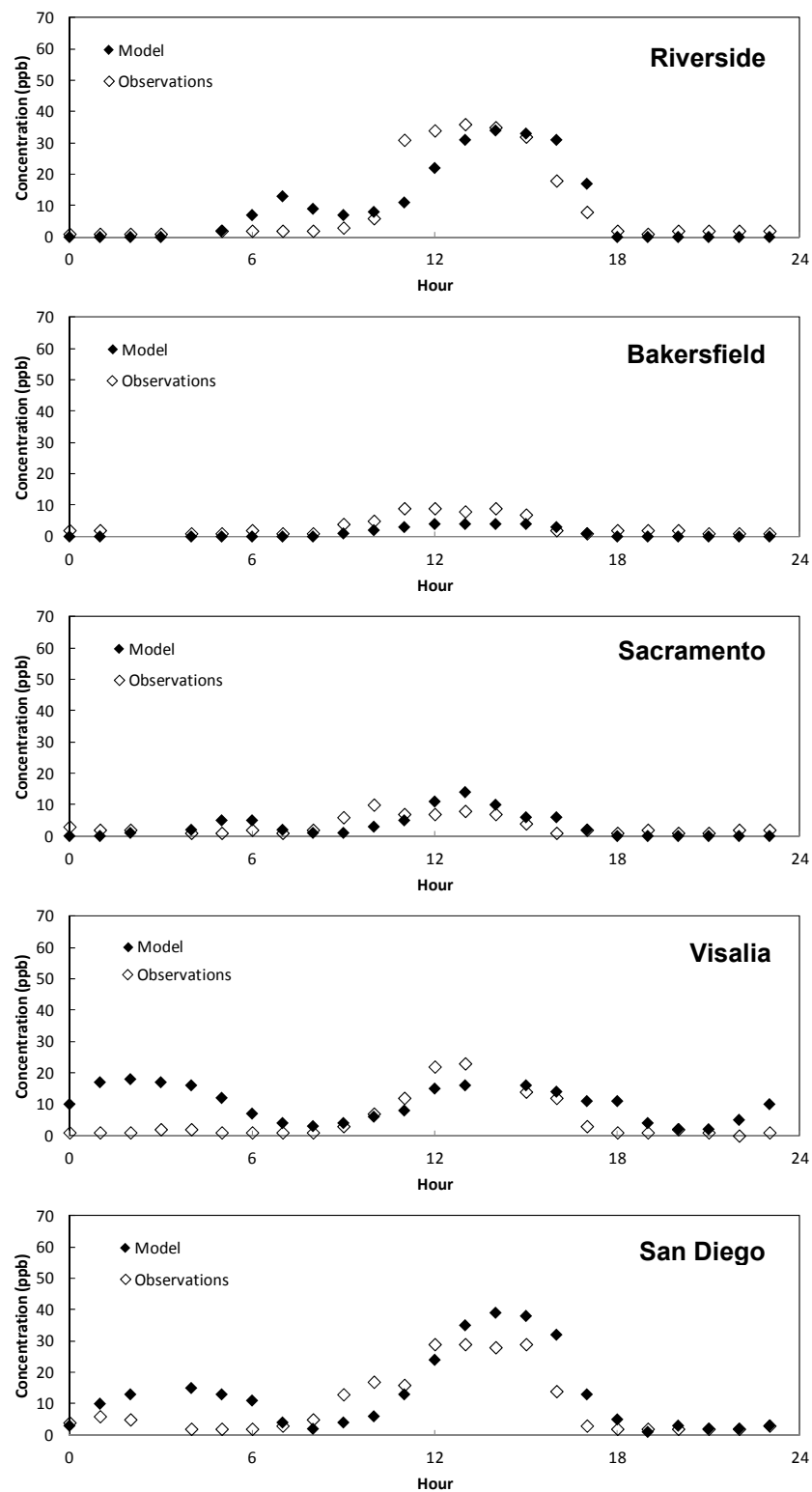
Figure 35: Modeled and observed hourly ozone concentrations for December 7, 2005 at selected locations
