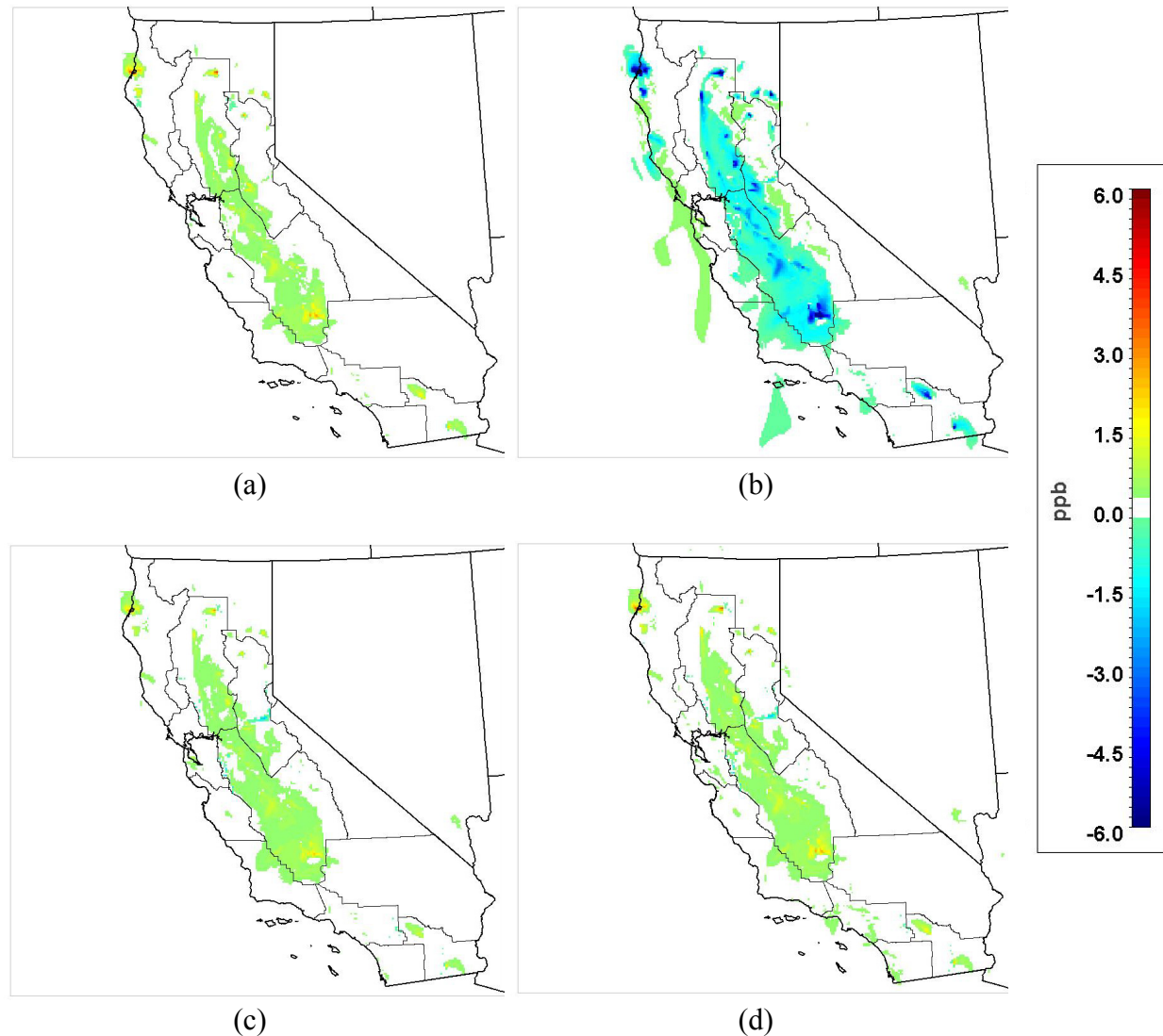
Figure 40: Changes in peak ozone concentrations due to biomass scenarios in a winter episode: (a) No Biomass Case, (b) Maximum biopower production with current technology (group A-4), (c) Maximum biopower production with enhanced technology (group B), (d) Maximum production of CNG from biomass (group C-1).
