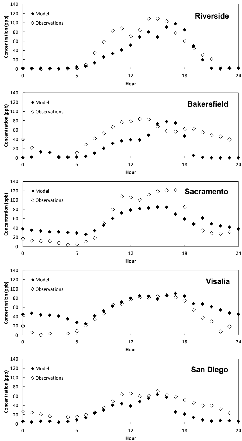
Figure 32: Modeled and observed hourly ozone concentrations for July 13, 2005 at selected locations
