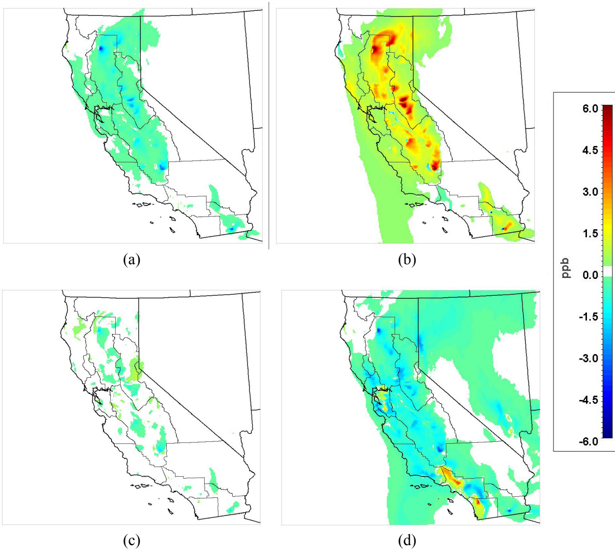
Figure 38: Changes in peak ozone concentrations due to biomass scenarios in a summer episode with respect to the baseline case: (a) No Biomass Case, (b) Maximum biopower production with current technology (group A-4), (c) Maximum biopower production with enhanced technology (group B), (d) Maximum production of CNG from biomass for vehicle consumption (group C-1).
