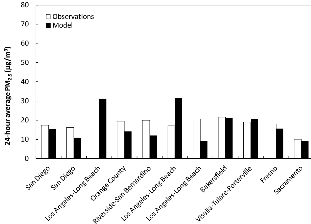
Figure 33: Modeled and observed 24-hour average PM 2.5 concentrations for July 13, 2005 at selected locations
