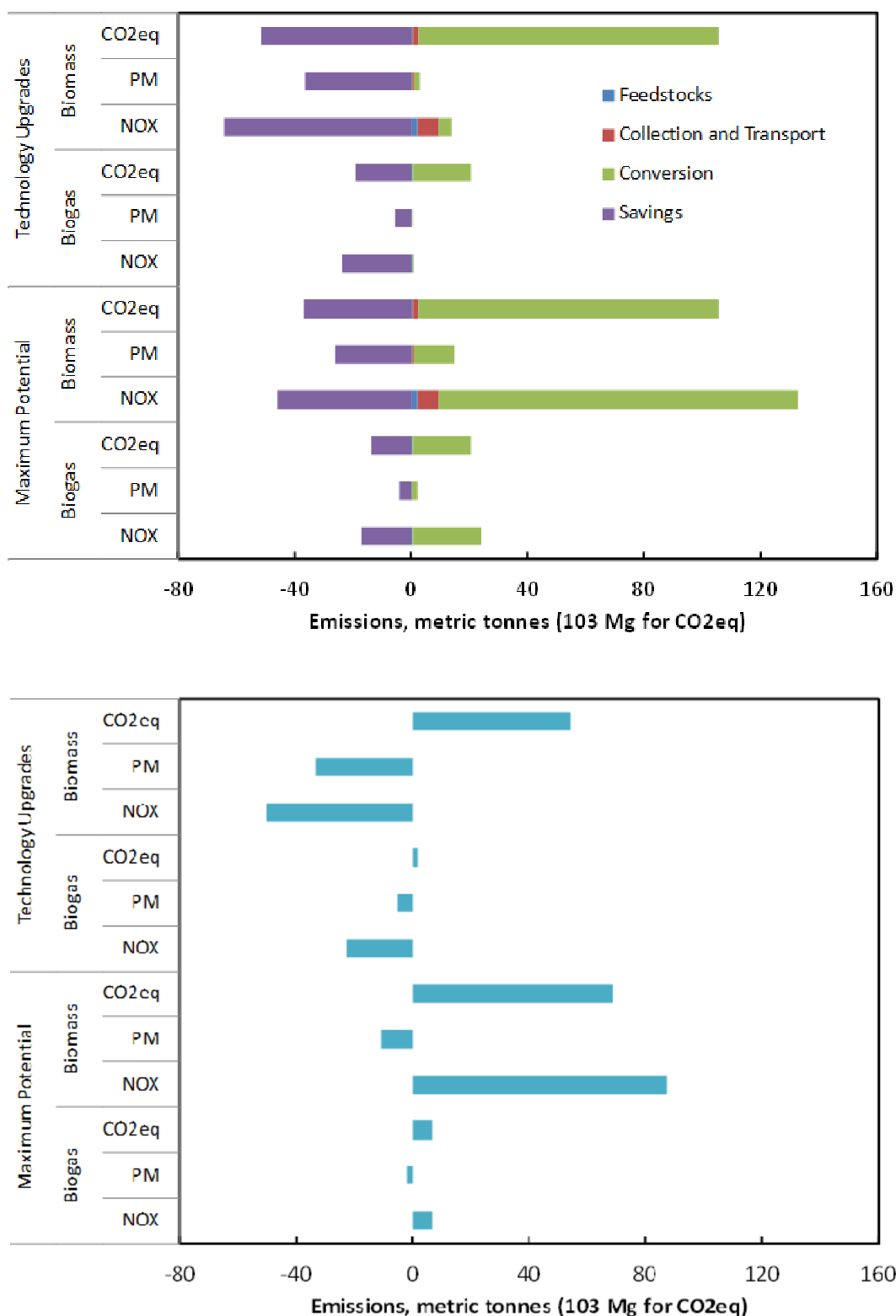
Figure ES2: Comparison of emissions from biomass in scenarios with maximum biomass technical potential with current technology (Group A-4) and with technology upgrades for efficiency and emissions (Group B). Top: all emissions; Bottom: net emissions
