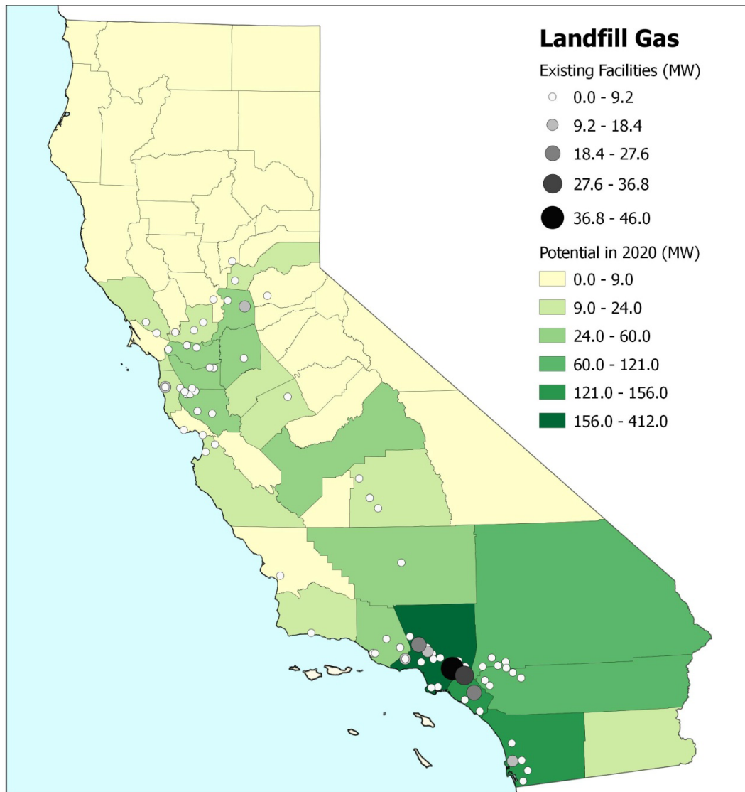
Figure 2: Landfill gas potential for biopower production in 2020 and capacity and location of existing facilities in California. Data on facilities from CBC, 2013; data on potential from Williams et al., 2008.
