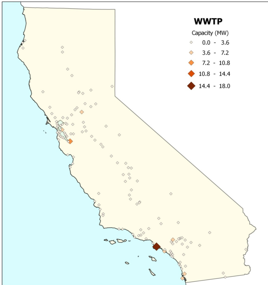
Figure 3: Capacity and location of existing biopower facilities in California in wastewater treatment plants (WWTP). Data on facilities from CBC, 2013.
