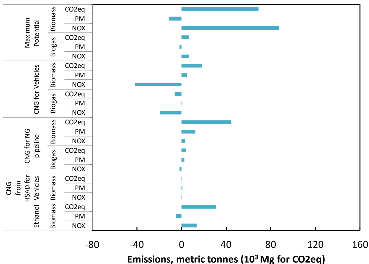
Figure 30: Comparison of emissions from biomass in scenarios with maximum biomass potential using current technology for biopower (group A) and scenarios with a shift end use from electricity to fuel (group C-1, C-2, C-3 and C-4)
