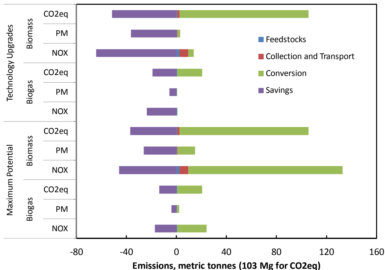
Figure 27: Comparison of emissions from biomass in scenarios with maximum biomass potential with current technology (group A-4) and with technology upgrades for efficiency and emissions (group B)
