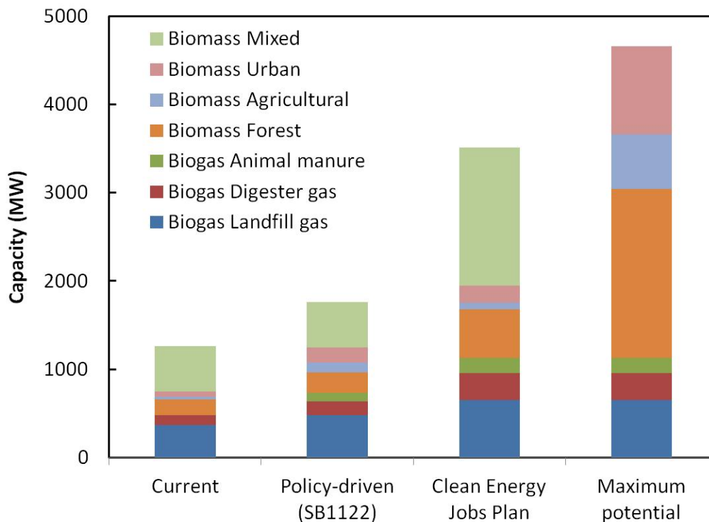
Figure ES1: Summary of power generation capacity from biomass scenarios with current biomass technology estimated for the year 2020
