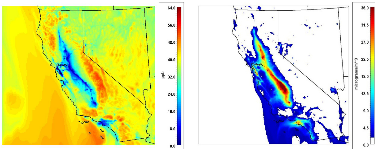
Figure 34: Modeled pollutant concentrations for December 7, 2005: (a) 8-hour average ozone, (b) 24-hour average PM 2.5 .
