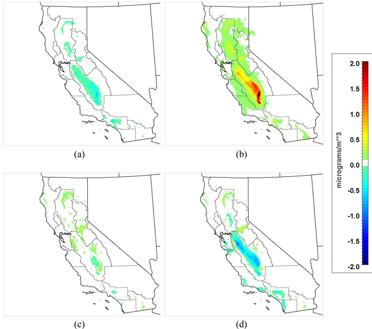
Figure 39: Changes in 24-hour average PM_{2.5} concentrations due to biomass scenarios in a summer episode: (a) No Biomass Case, (b) Maximum biopower production with current technology (group A-4), (c) Maximum biopower production with enhanced technology (group B), (d) Maximum production of CNG from biomass (group C-1).
