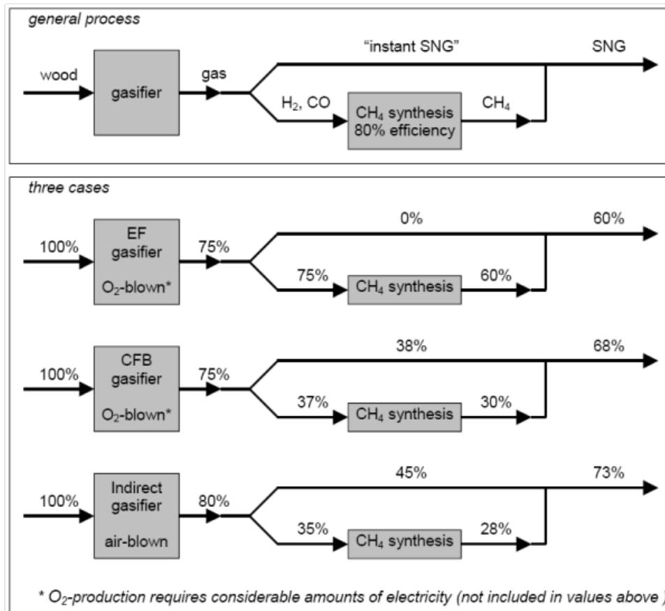
Figure 23: SNG production efficiencies for different gasification technologies (From Zwart et al., 2006)
