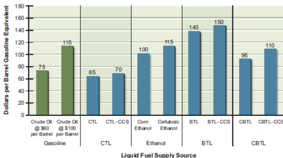
Figure 20: Estimated gasoline-equivalent costs of alternative liquid fuels in 2007 dollars. Note: BTL=biomass-to-liquid; CBTL=coal-and-biomass-to-liquid; CTL= coal-to-liquid fuel Source: NRC 2009
