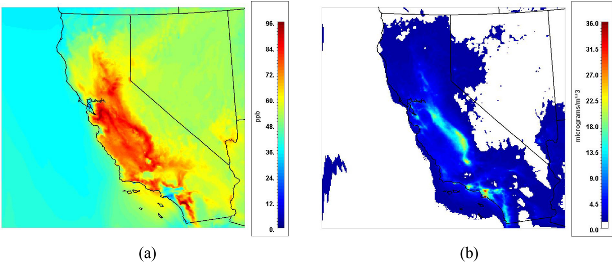
Figure 31: Ambient air concentrations for July 13, 2005: (a) 8-hour average ozone, (b) 24-hour average PM 2.5 .
