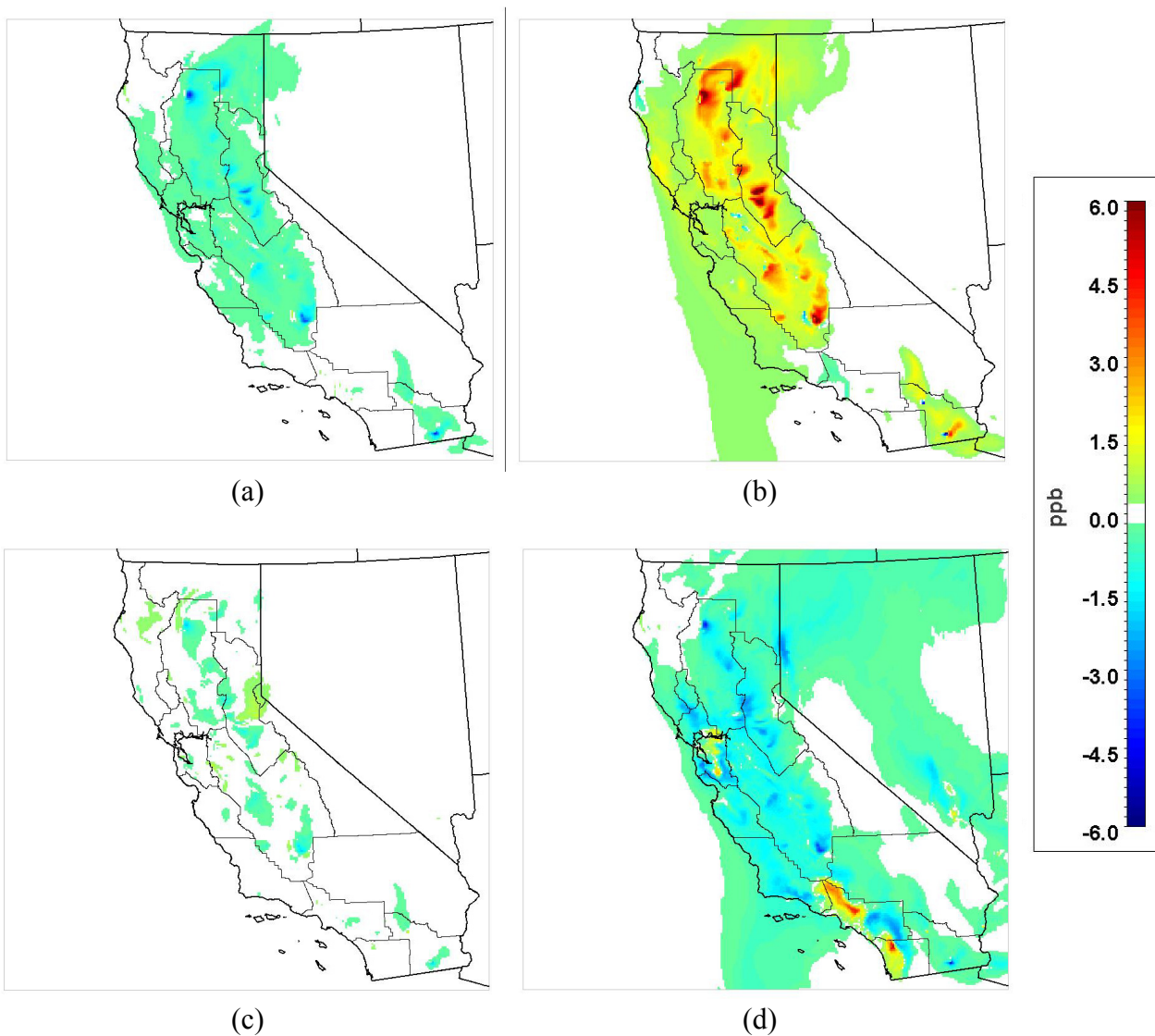
Figure ES5: Changes in peak ozone concentrations due to biomass scenarios in a summer episode with respect to the ‘Current biopower capacity’ case: (a) No Biomass Case, (b) Maximum biopower production with current technology (group A-4), (c) Maximum biopower production with enhanced technology (group B), (d) Maximum production of CNG from biomass for vehicle consumption (group C-1).
