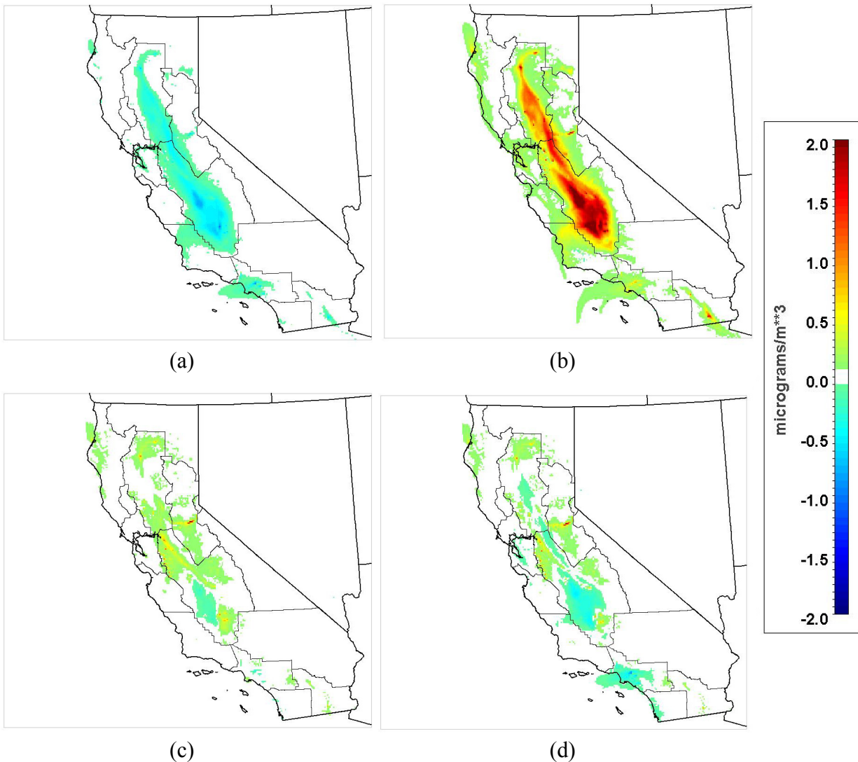
Figure 41: Changes in 24-hour average PM 2.5 concentrations due to biomass scenarios in a winter episode: (a) No Biomass Case, (b) Maximum biopower production with current technology (group A-4), (c) Maximum biopower production with enhanced technology (group B), (d) Maximum production of CNG from biomass (group C-4).
